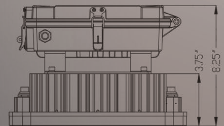
Dimensions Schematic
